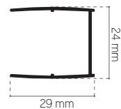
profilo murale profilé mural_wall profile
