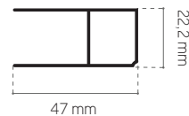
profilo murale profilé mural_wall profile
