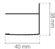
profilo murale profilé mural_wall profile
